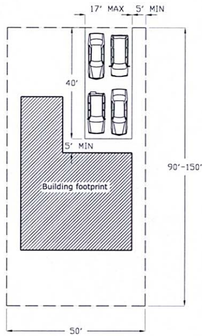
OPTION II - TANDEM PARKING - 4 CARS
