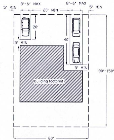
OPTION II - SPLIT PARKING - 3 CARS
