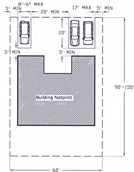
OPTION III - SPLIT PARKING - 3 CARS (PERMITTED ONLY IF TANDEM PARKING NOT AVAILABLE)
