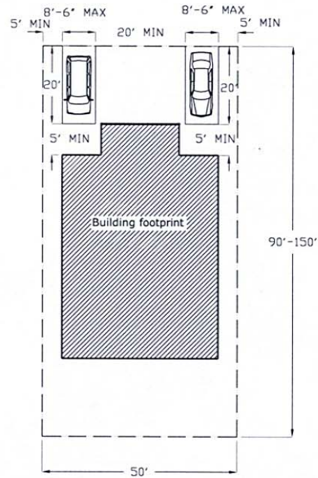
OPTION III - SPLIT PARKING (PERMITTED ONLY IF TANDEM PARKING NOT AVAILABLE)
