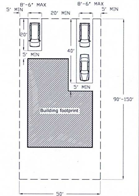
OPTION IV - SPLIT & TANDEM PARKING
