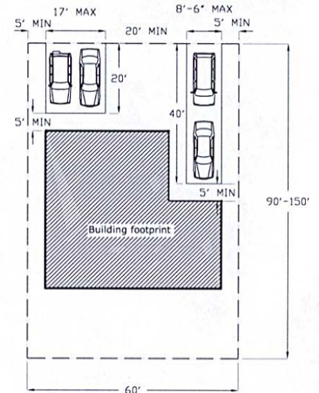
OPTION IV - SPLIT & TANDEM PARKING
